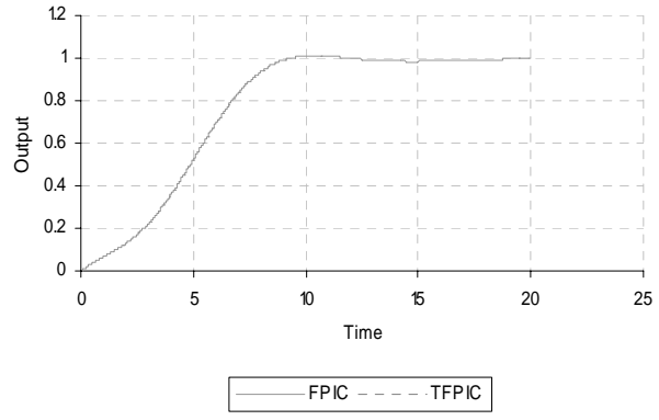
Fig. 11. Response of nonlinear system with FPIC.
